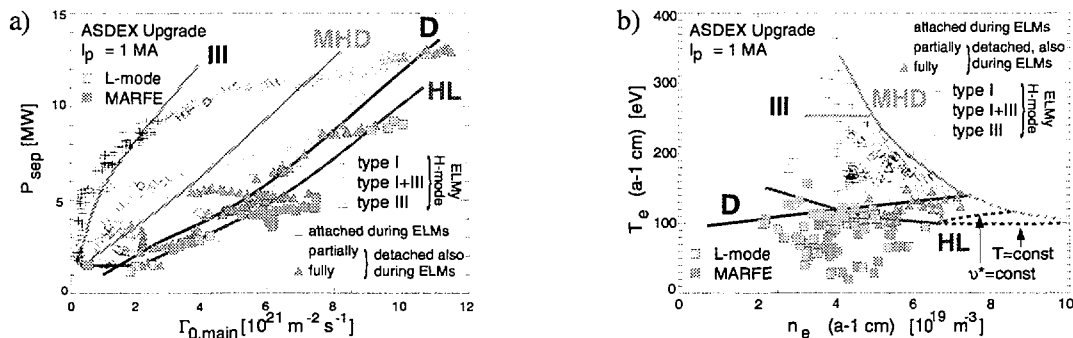
Figure 2: Operational space at high edge densities: a) separatrix power and main chamber neutral gas flux, b) edge density and edge temperature (taken at r = a - 1 \text{ cm} ). Regime boundaries marked “III”, “MHD”, “D”, and “HL” are discussed in the text.
