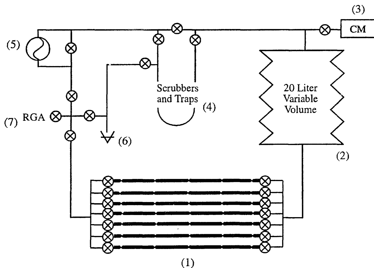
Figure 8: Gas isotope standard production system. (1) Set of seven parallel glass lines, prepinned into several open breakseals; valves are driven by pneumatic solenoids; (2) 20 liter stainless steel variable volume; (3) Capacitance manometer; (4) Scrubbers and traps for gas purification; (5) Metal bellows pump; (6) Vacuum system - molecular drag pump; (7) Gas inlet and residual gas analyzer. See section 3.1.
