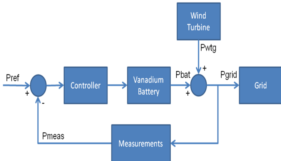
Figure 23 Setup for smoothing controller
