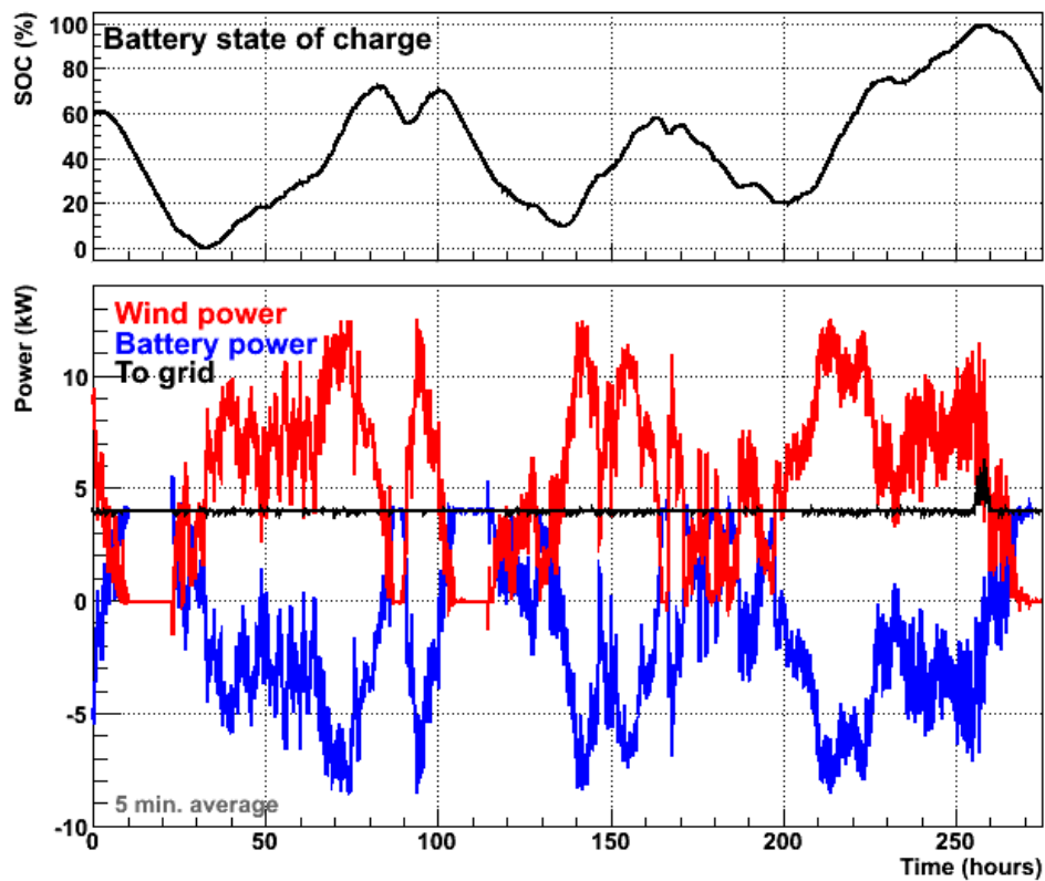
Figure 24 Vanadium battery operated to smooth output from wind turbine (11kW Gaia wind turbine)
