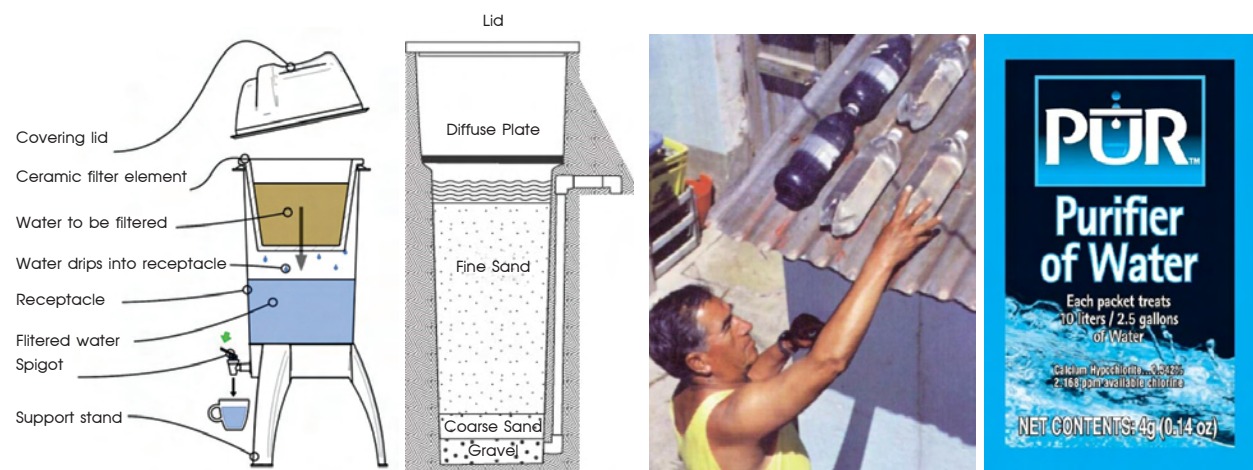
Figure 5: Cross-sections and photographs of four popular POU technologies. On the left are two popular POU filters with descriptions of the individual elements; the ceramic water purifier (on the far left) and a concrete biosand water filter (BSF) (second from left). Both of the devices pictured stand between 0.5-1 meter high. Second from the right is a photo of bottles used for solar disinfection (SODIS) being placed on a household roof. On the far right is an image of a Procter & Gamble PUR coagulation/chlorination packet; an individual packets contains 4 g of crystals and can be used to treat 10 liters of water.
