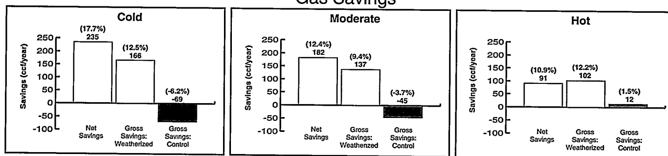
Gas Savings by Climate Region.
