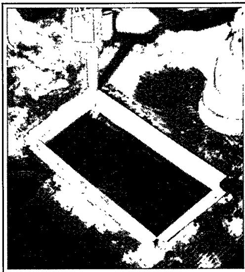
The interface between the riser in a supply duct and the floor of a mobile home is frequently found to be a source of air leaks, both when the furnace fan is on and when it is not. Here a technician in Indiana uses a technique his agency developed to achieve a tight, lifelong seal.
